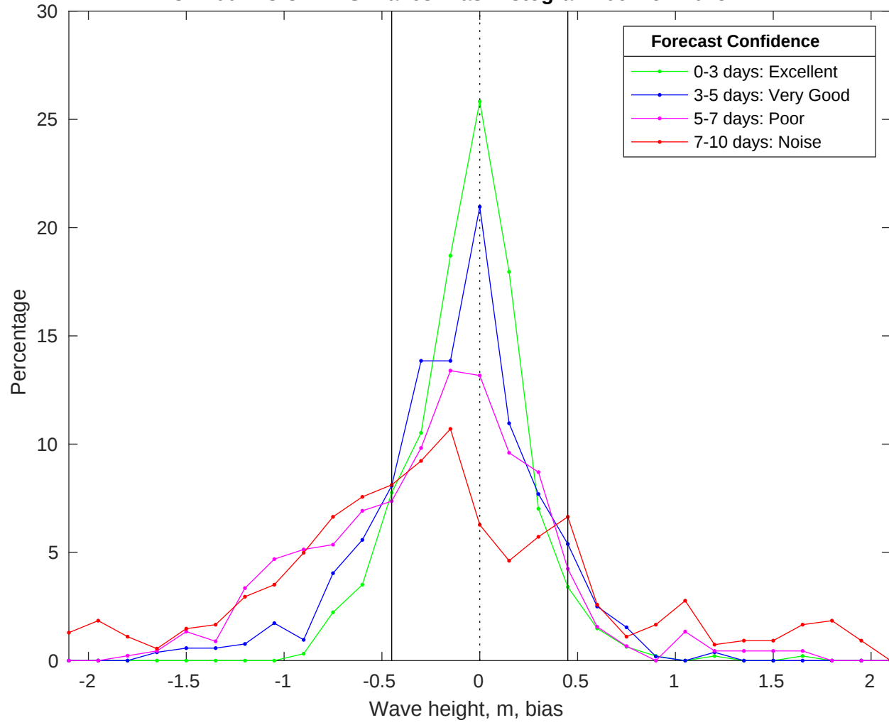
NDBC 41004 vs CMEMS Waves Bias Histogram: 06-Nov-2025
