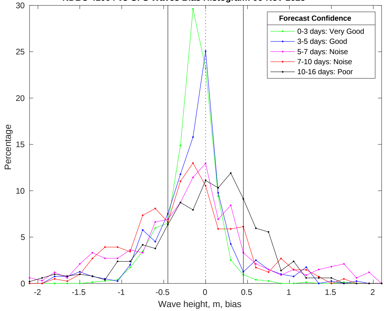
NDBC 41004 vs GFS Waves Bias Histogram: 06-Nov-2025
