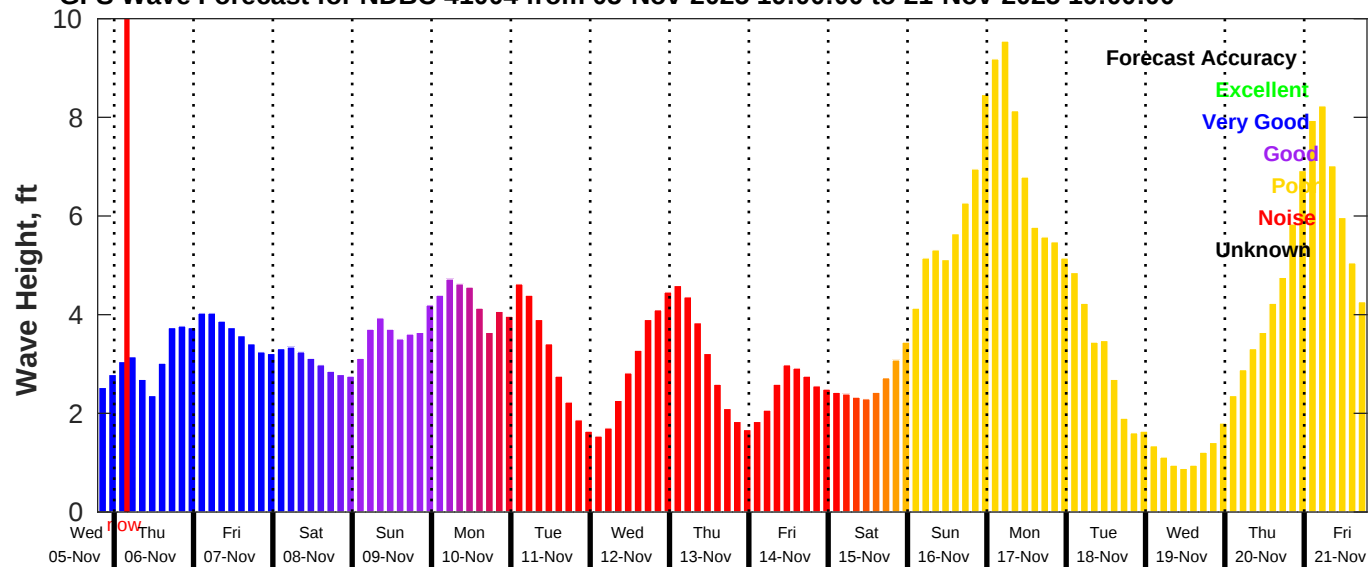
GFS Wave Forecast for NDBC 41004 from 05-Nov-2025 19:00:00 to 21-Nov-2025 19:00:00
