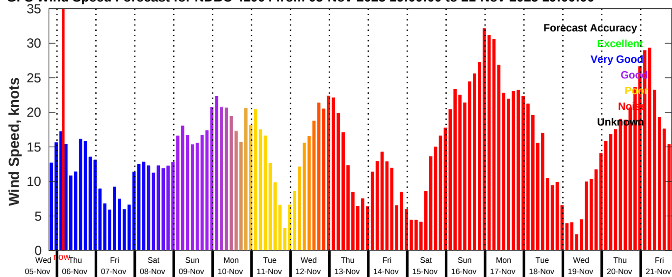
GFS Wind Speed Forecast for NDBC 41004 from 05-Nov-2025 19:00:00 to 21-Nov-2025 19:00:00
