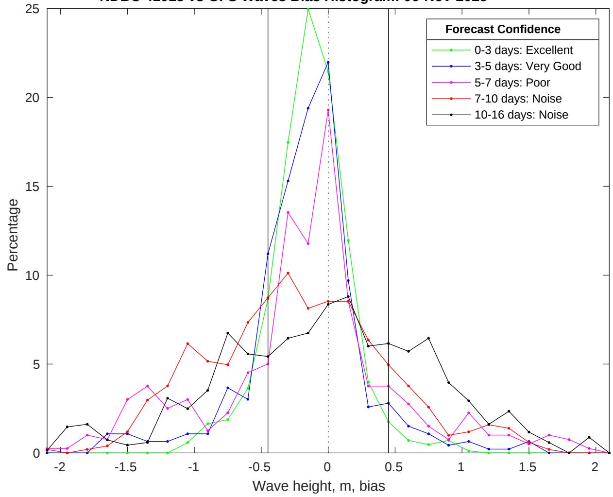
NDBC 41013 vs GFS Waves Bias Histogram: 06-Nov-2025
