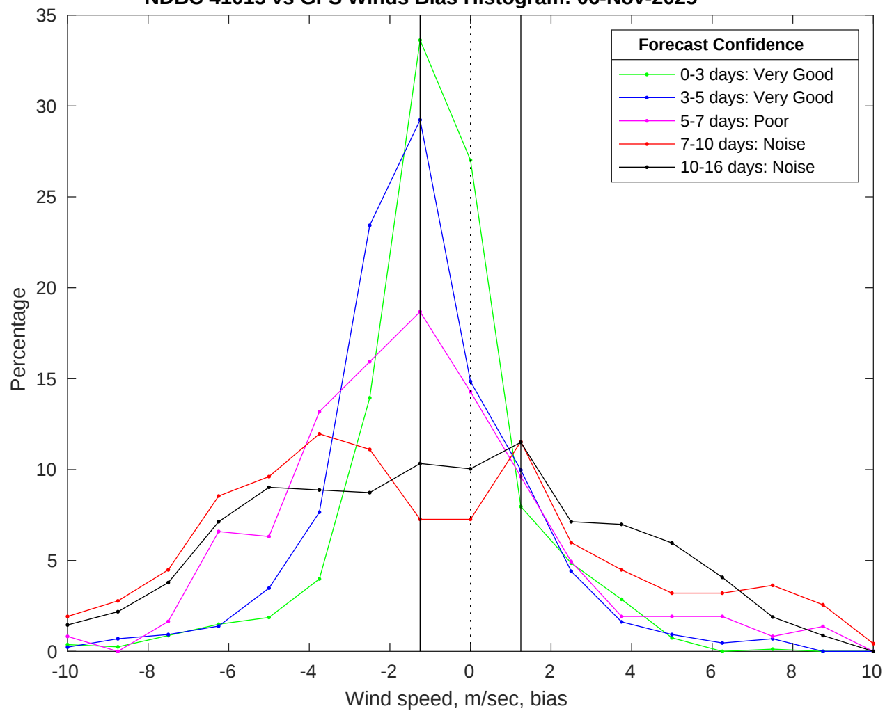
NDBC 41013 vs GFS Winds Bias Histogram: 06-Nov-2025
