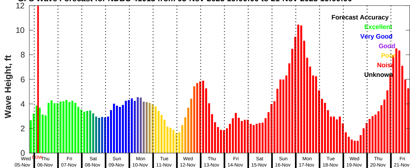
GFS Wave Forecast for NDBC 41013 from 05-Nov-2025 19:00:00 to 21-Nov-2025 19:00:00
