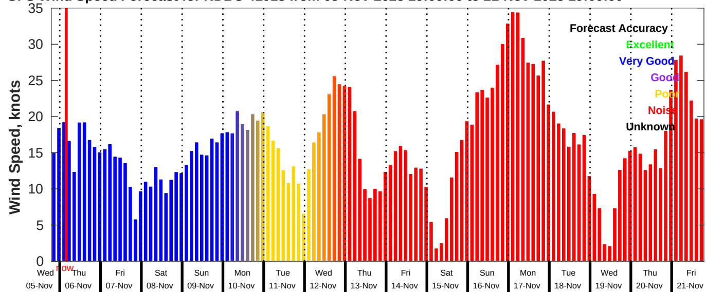
GFS Wind Speed Forecast for NDBC 41013 from 05-Nov-2025 19:00:00 to 21-Nov-2025 19:00:00
