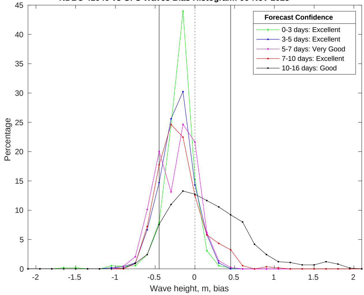
NDBC 41040 vs GFS Waves Bias Histogram: 06-Nov-2025
