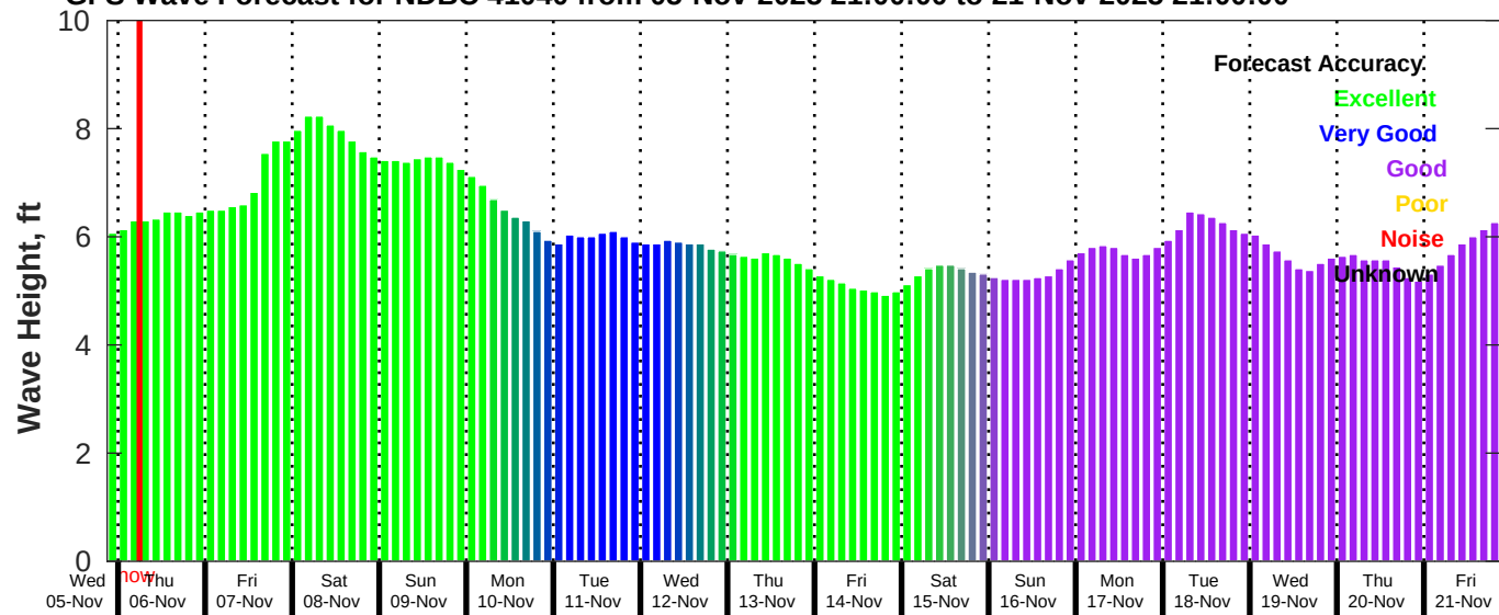
GFS Wave Forecast for NDBC 41040 from 05-Nov-2025 21:00:00 to 21-Nov-2025 21:00:00
