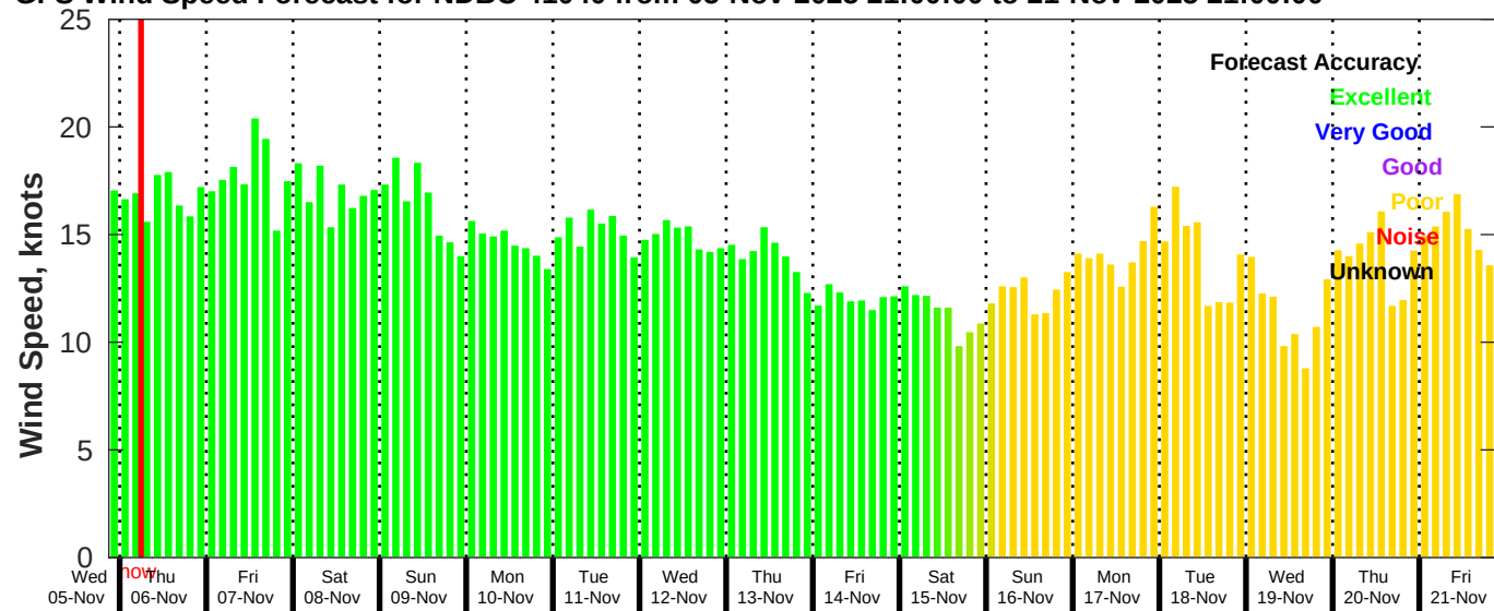
GFS Wind Speed Forecast for NDBC 41040 from 05-Nov-2025 21:00:00 to 21-Nov-2025 21:00:00
