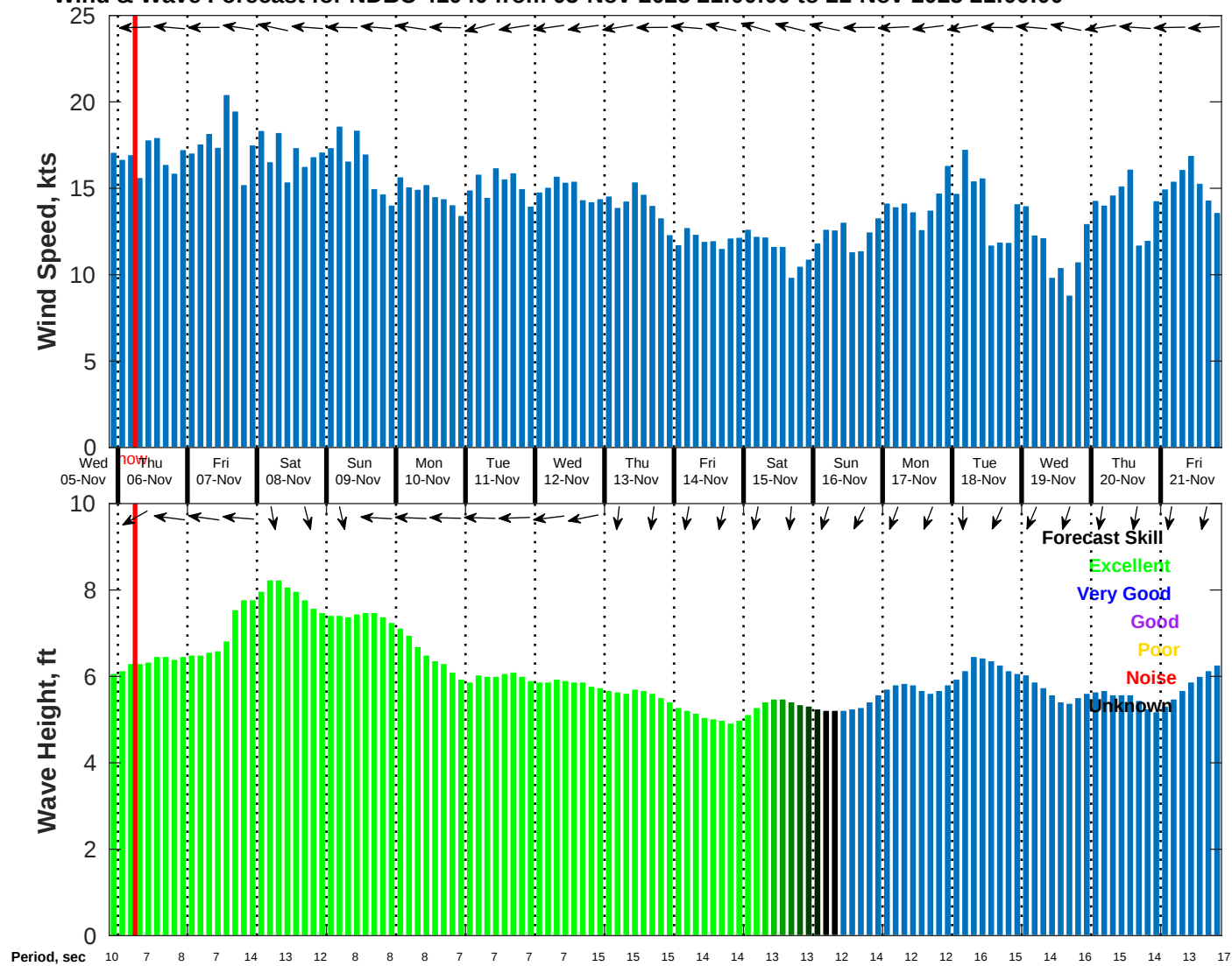
Wind & Wave Forecast for NDBC 41040 from 05-Nov-2025 21:00:00 to 21-Nov-2025 21:00:00
