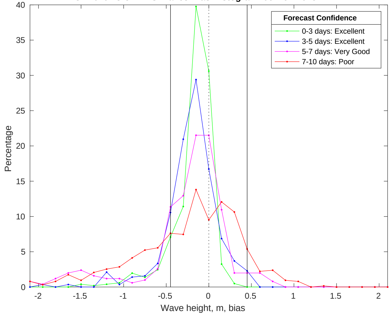
NDBC 42019 vs CMEMS Waves Bias Histogram: 06-Nov-2025
