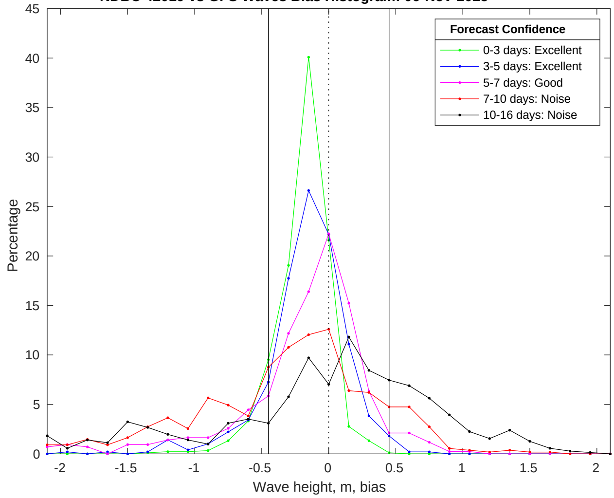
NDBC 42019 vs GFS Waves Bias Histogram: 06-Nov-2025
