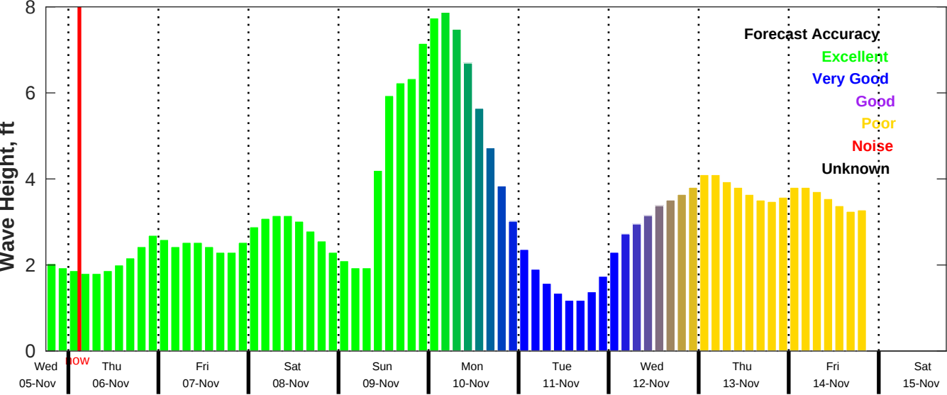
CMEMS Wave Forecast for NDBC 42019 from 05-Nov-2025 18:00:00 to 15-Nov-2025 18:00:00
