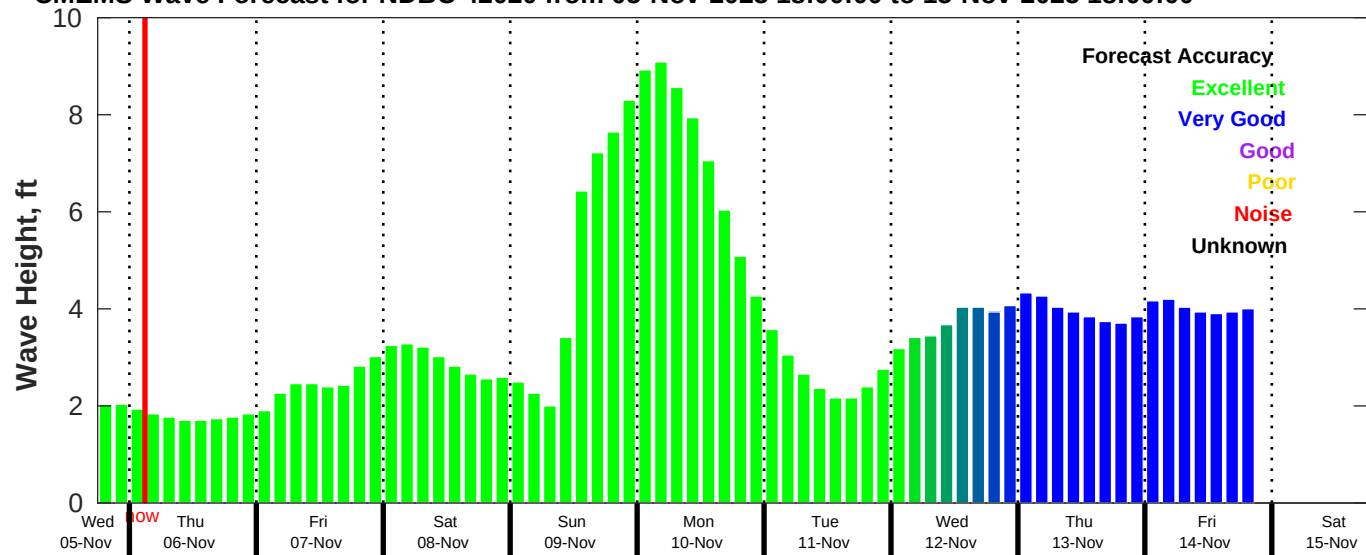
CMEMS Wave Forecast for NDBC 42020 from 05-Nov-2025 18:00:00 to 15-Nov-2025 18:00:00
