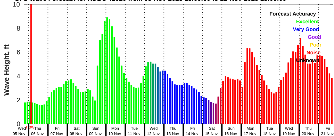
GFS Wave Forecast for NDBC 42020 from 05-Nov-2025 18:00:00 to 21-Nov-2025 18:00:00
