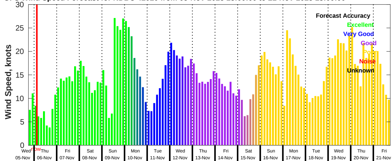
GFS Wind Speed Forecast for NDBC 42020 from 05-Nov-2025 18:00:00 to 21-Nov-2025 18:00:00
