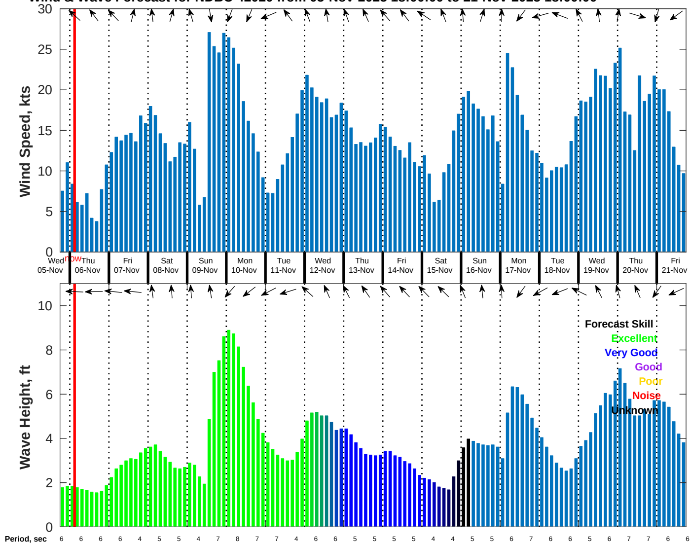
Wind & Wave Forecast for NDBC 42020 from 05-Nov-2025 18:00:00 to 21-Nov-2025 18:00:00
