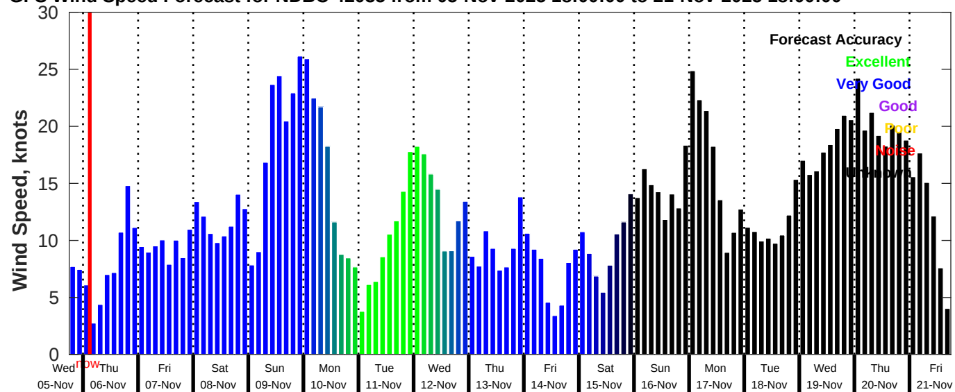
GFS Wind Speed Forecast for NDBC 42035 from 05-Nov-2025 18:00:00 to 21-Nov-2025 18:00:00
