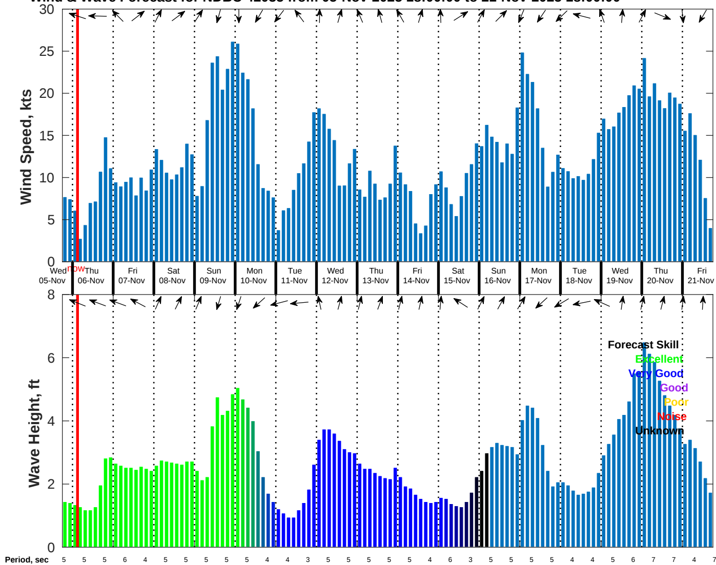
Wind & Wave Forecast for NDBC 42035 from 05-Nov-2025 18:00:00 to 21-Nov-2025 18:00:00
