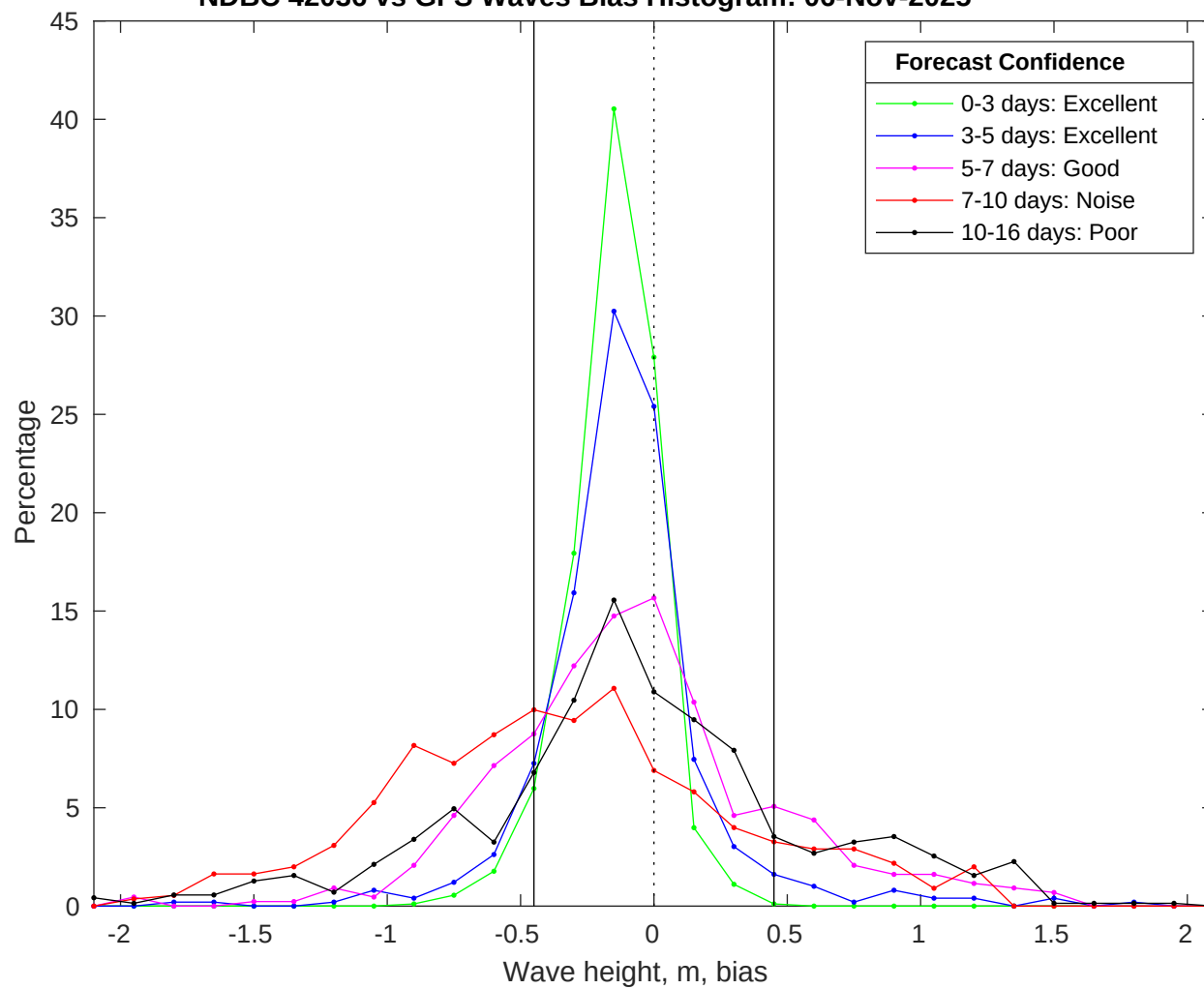
NDBC 42036 vs GFS Waves Bias Histogram: 06-Nov-2025
