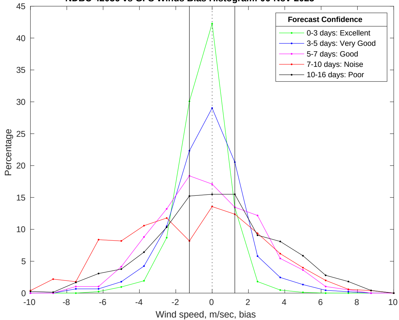
NDBC 42036 vs GFS Winds Bias Histogram: 06-Nov-2025
