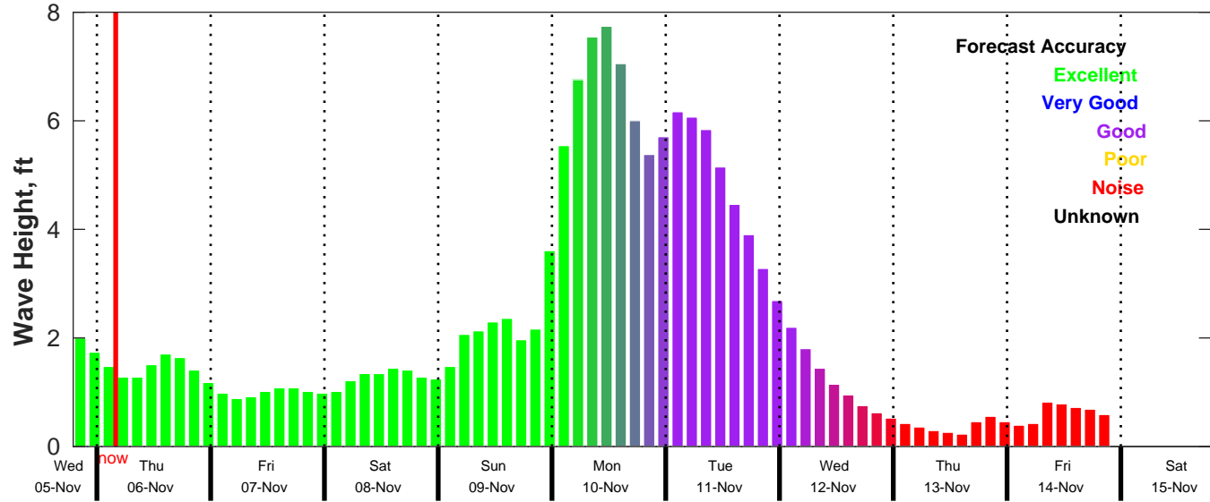
CMEMS Wave Forecast for NDBC 42036 from 05-Nov-2025 19:00:00 to 15-Nov-2025 19:00:00
