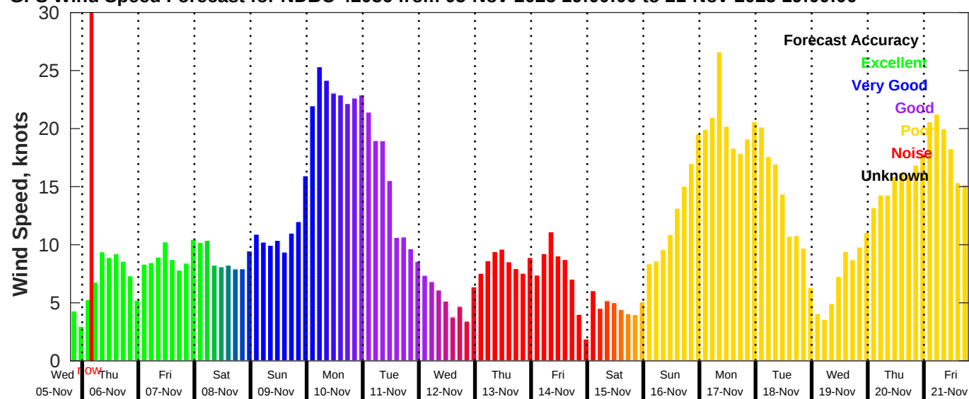
GFS Wind Speed Forecast for NDBC 42036 from 05-Nov-2025 19:00:00 to 21-Nov-2025 19:00:00
