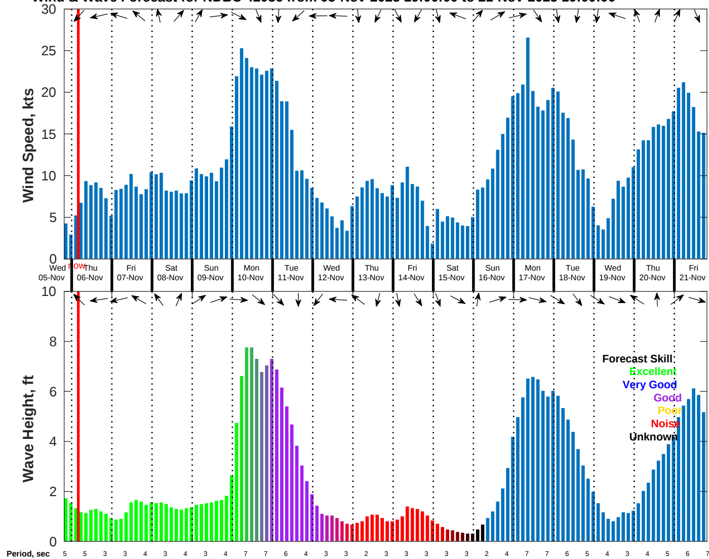
Wind & Wave Forecast for NDBC 42036 from 05-Nov-2025 19:00:00 to 21-Nov-2025 19:00:00
