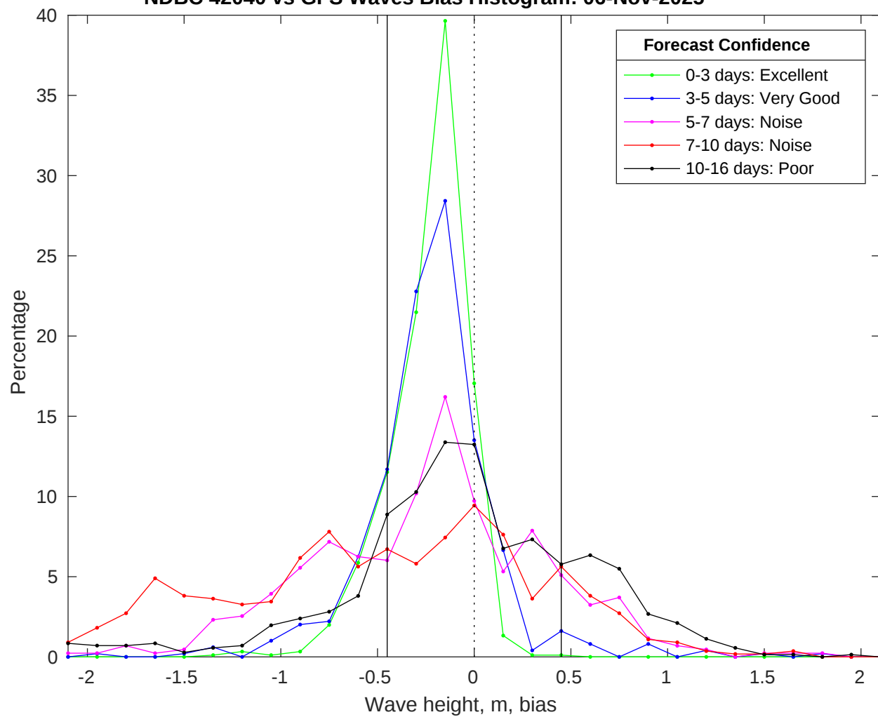
NDBC 42040 vs GFS Waves Bias Histogram: 06-Nov-2025
