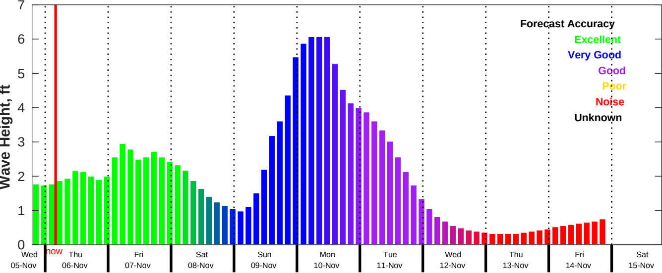
CMEMS Wave Forecast for NDBC 42040 from 05-Nov-2025 19:00:00 to 15-Nov-2025 19:00:00
