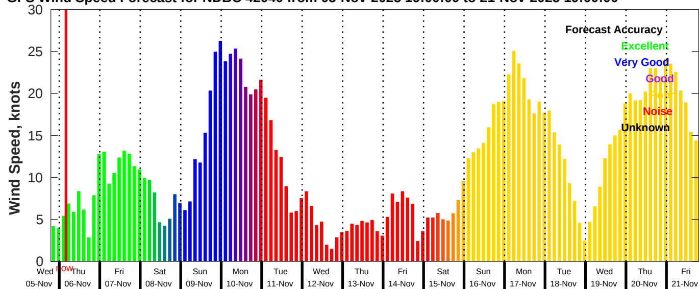
GFS Wind Speed Forecast for NDBC 42040 from 05-Nov-2025 19:00:00 to 21-Nov-2025 19:00:00
