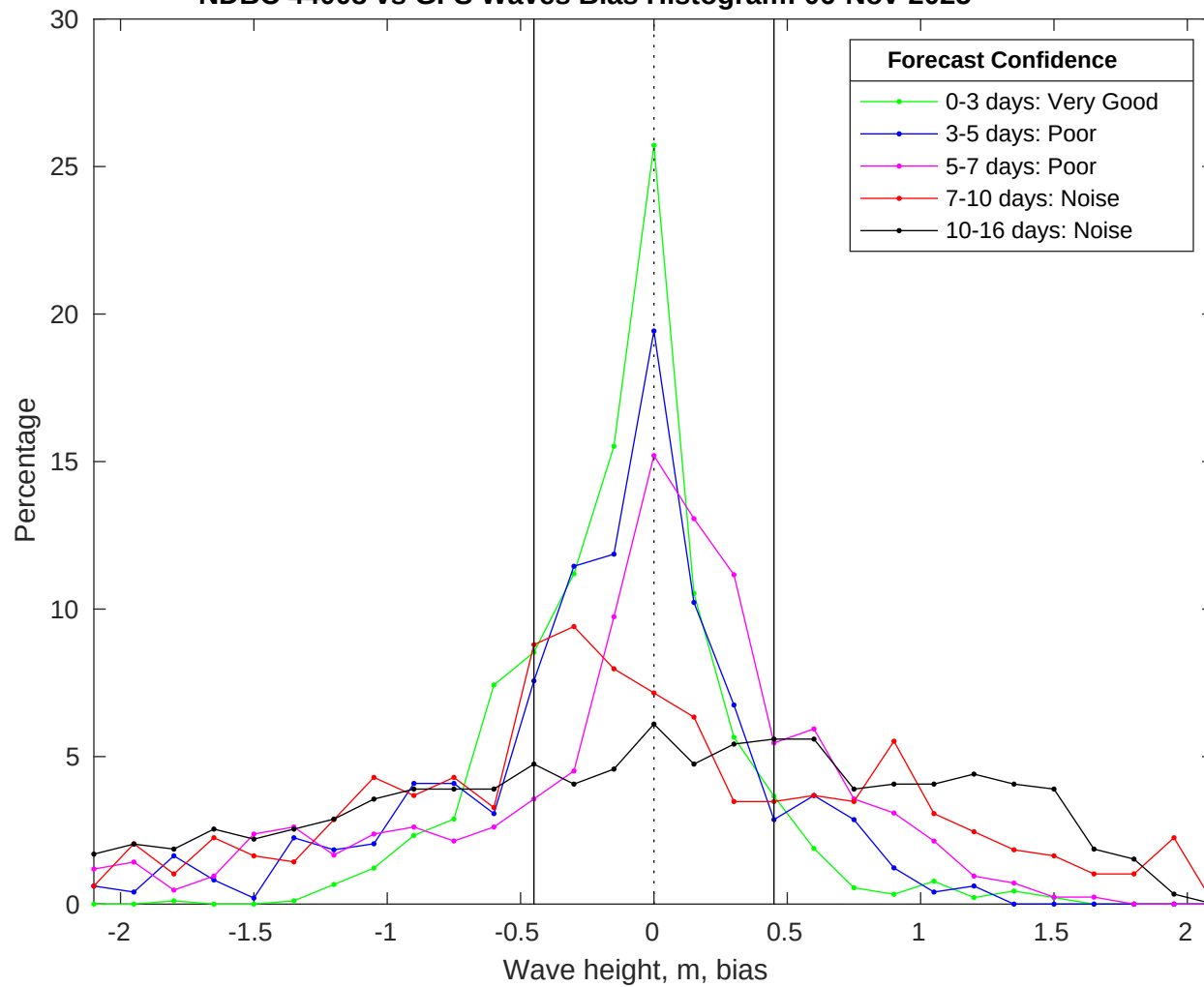
NDBC 44008 vs GFS Waves Bias Histogram: 06-Nov-2025
