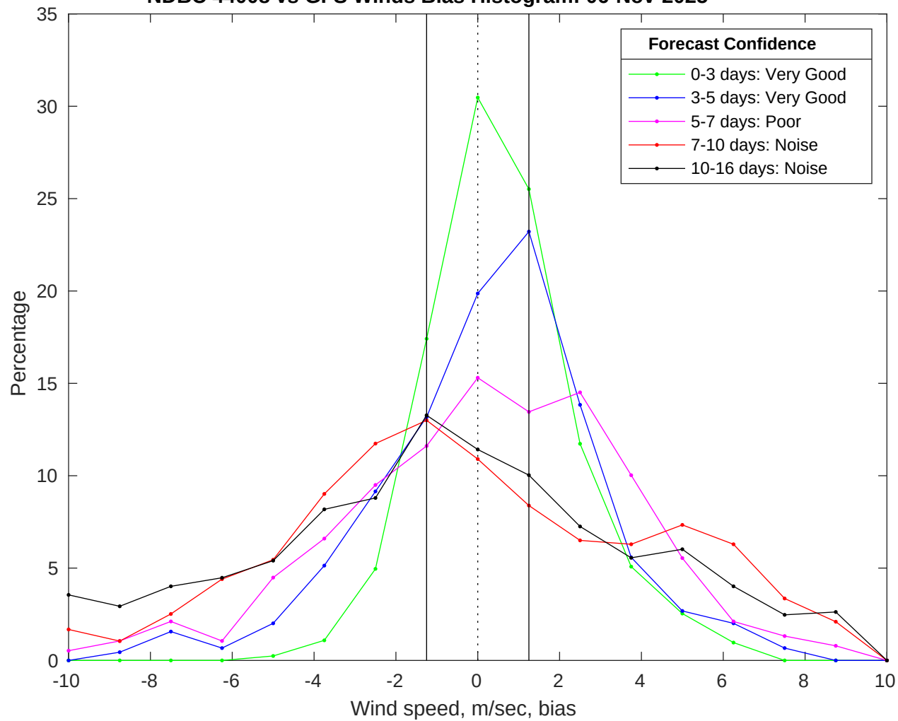
NDBC 44008 vs GFS Winds Bias Histogram: 06-Nov-2025
