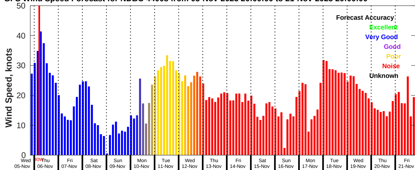
GFS Wind Speed Forecast for NDBC 44008 from 05-Nov-2025 20:00:00 to 21-Nov-2025 20:00:00
