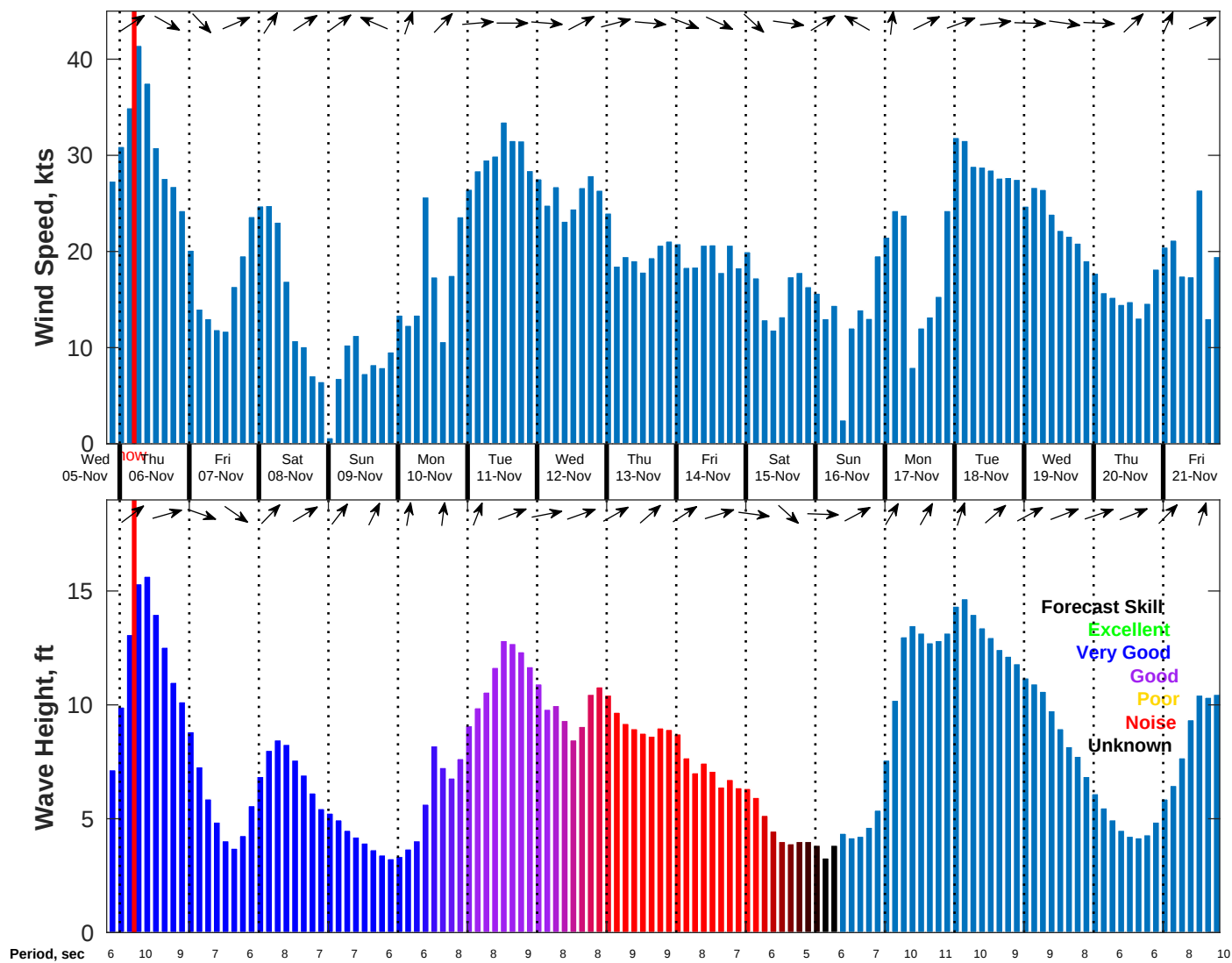
Wind & Wave Forecast for NDBC 44008 from 05-Nov-2025 20:00:00 to 21-Nov-2025 20:00:00
