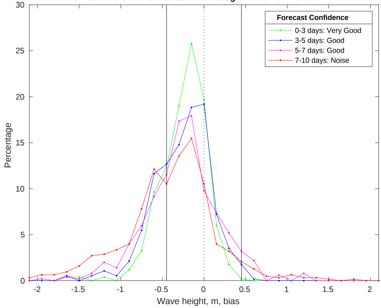
NDBC 46011 vs CMEMS Waves Bias Histogram: 06-Nov-2025
