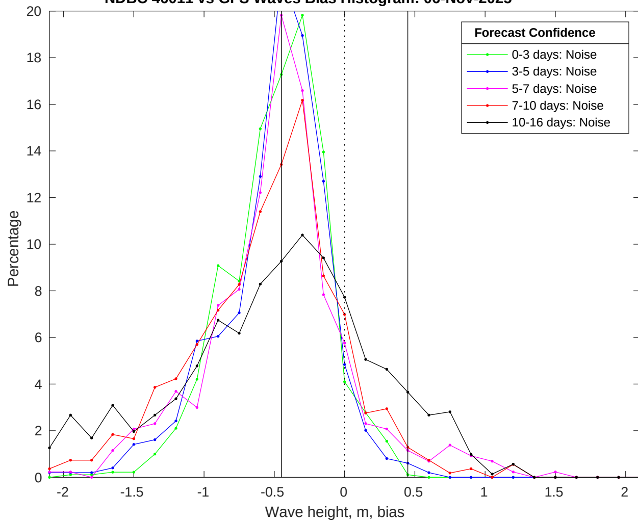
NDBC 46011 vs GFS Waves Bias Histogram: 06-Nov-2025
