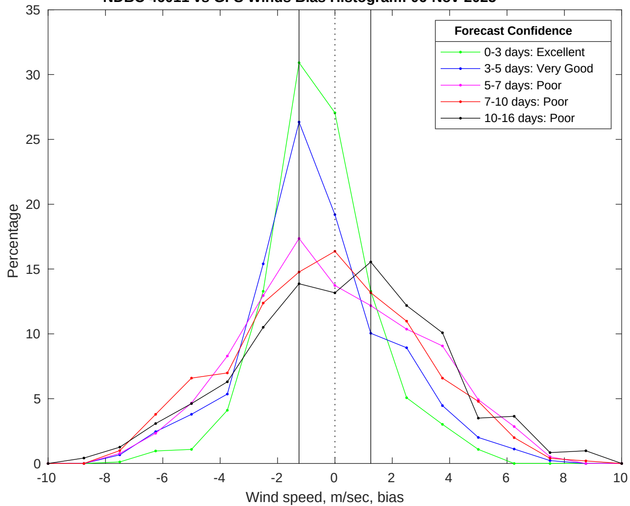
NDBC 46011 vs GFS Winds Bias Histogram: 06-Nov-2025
