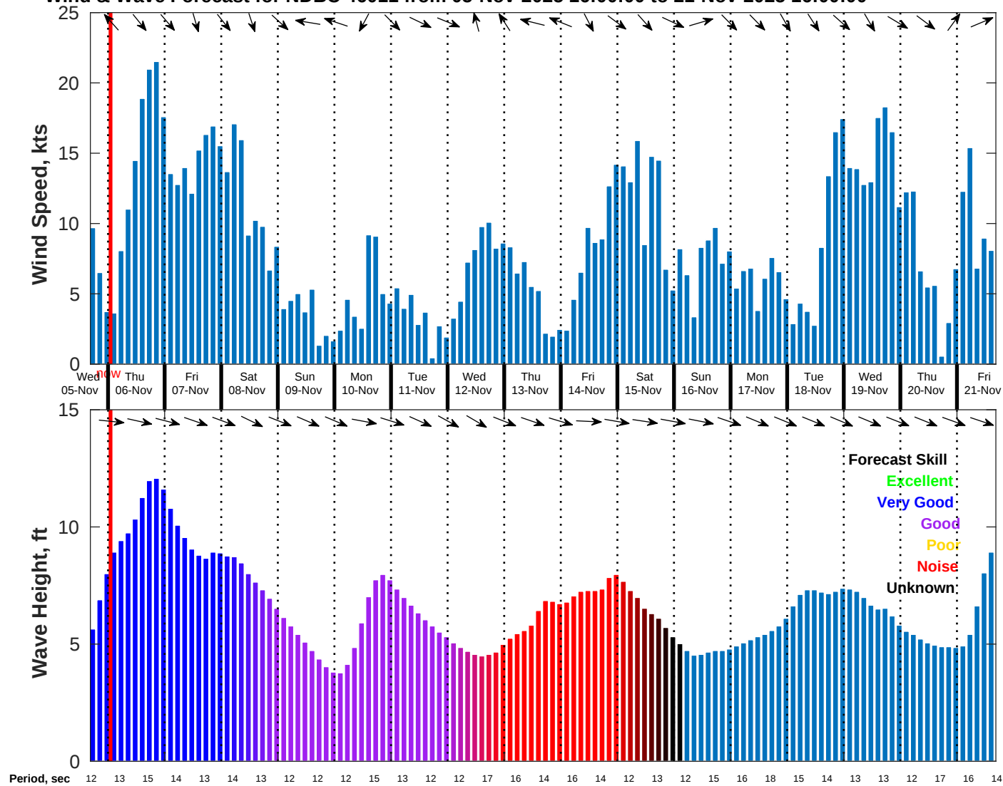
Wind & Wave Forecast for NDBC 46011 from 05-Nov-2025 16:00:00 to 21-Nov-2025 16:00:00
