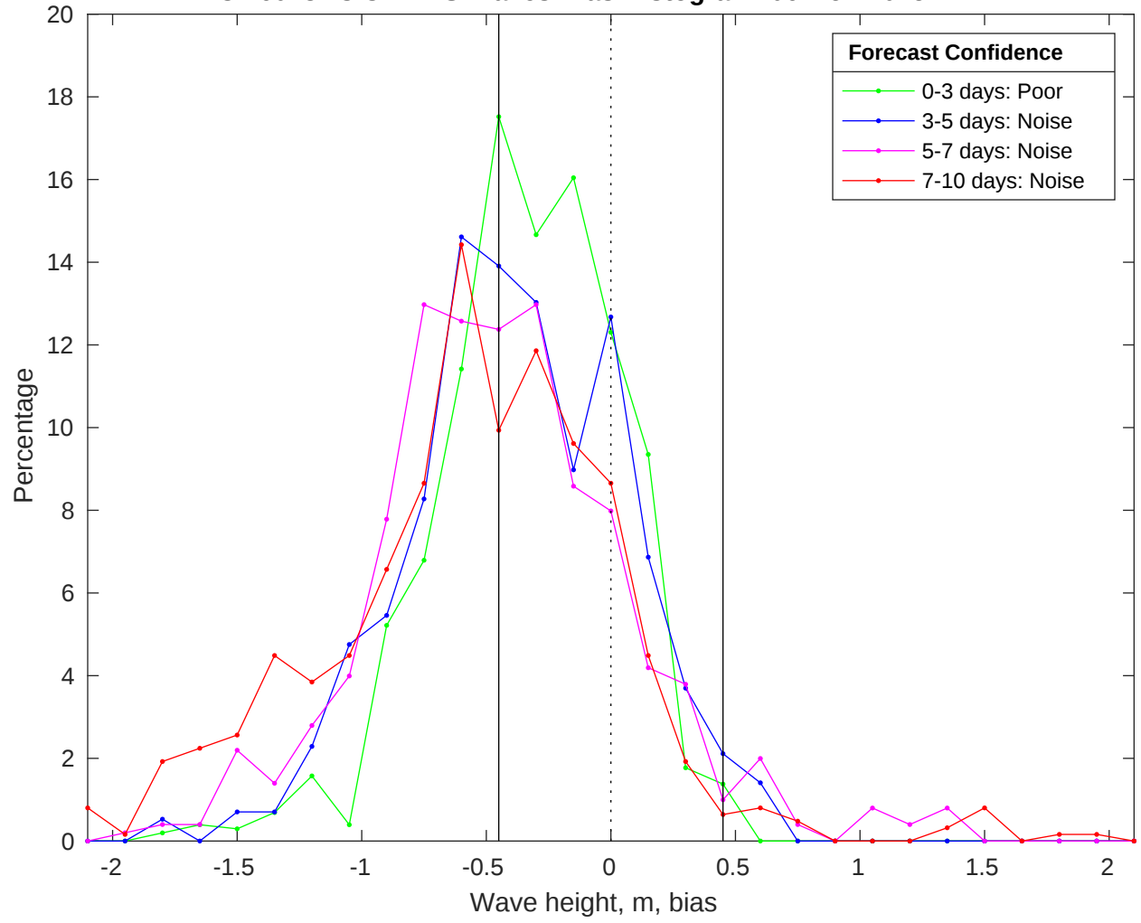
NDBC 46028 vs CMEMS Waves Bias Histogram: 06-Nov-2025
