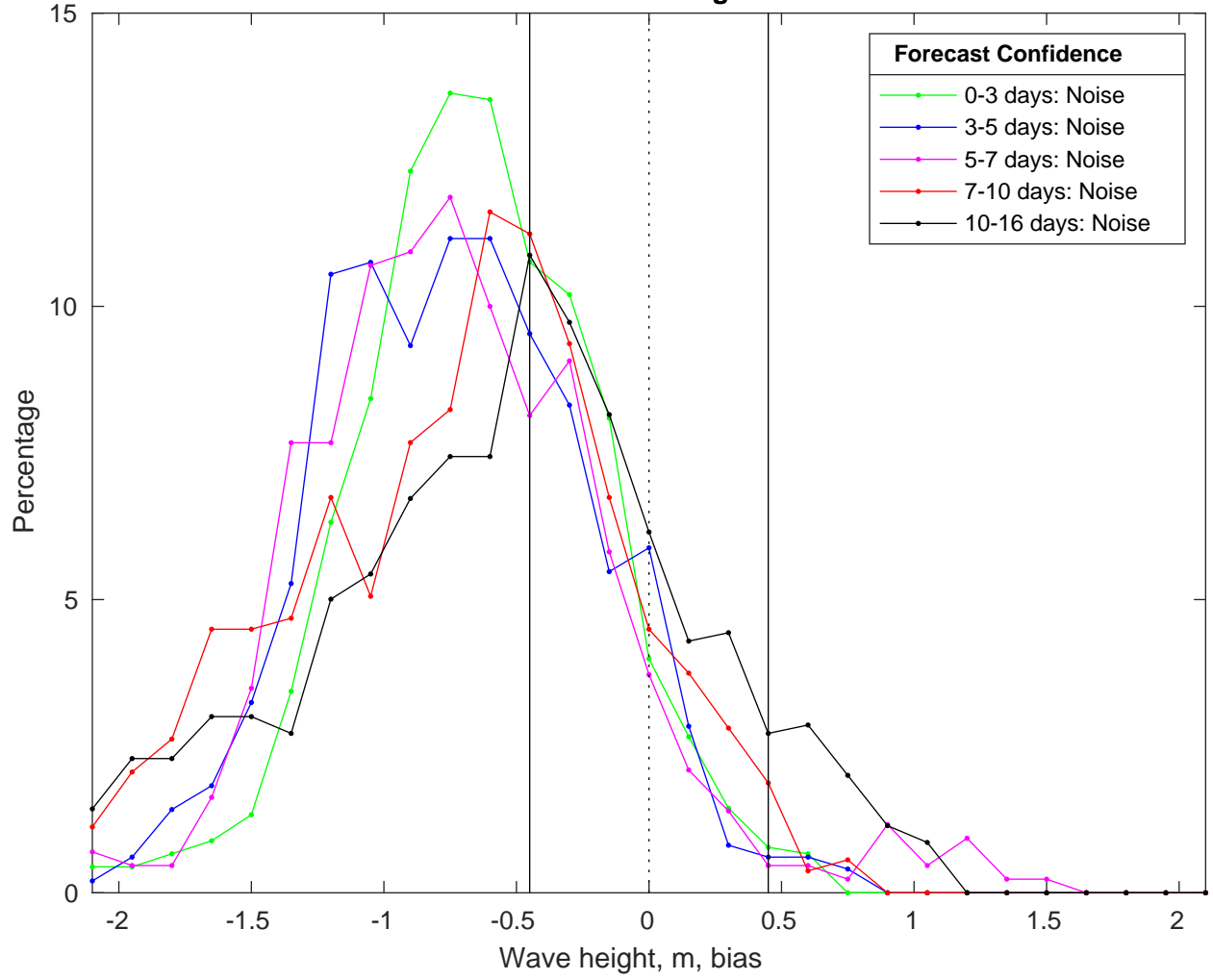
NDBC 46028 vs GFS Waves Bias Histogram: 06-Nov-2025
