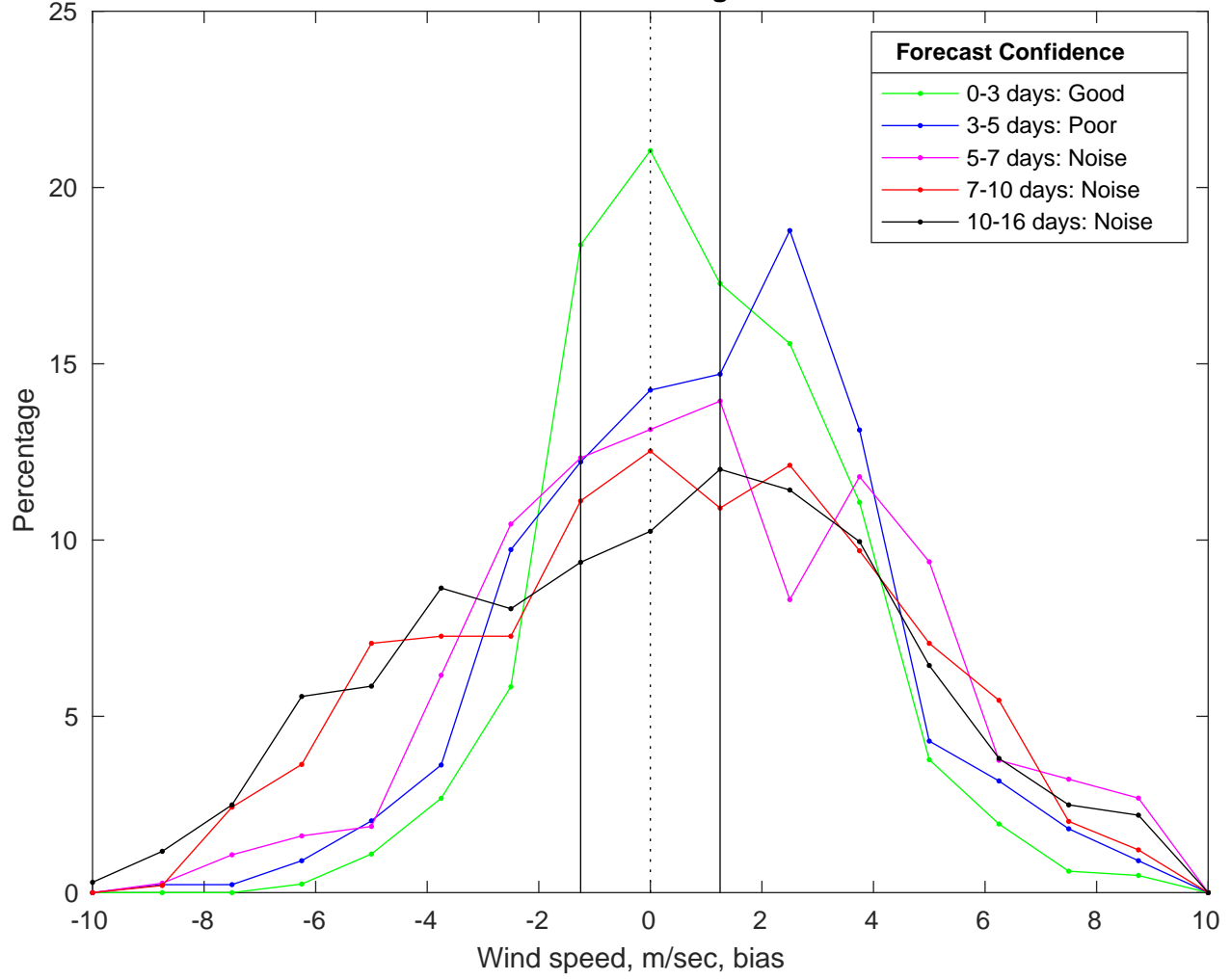
NDBC 46028 vs GFS Winds Bias Histogram: 06-Nov-2025
