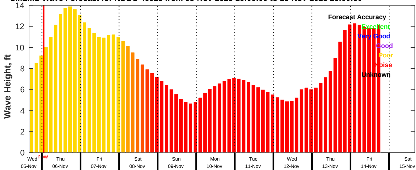
CMEMS Wave Forecast for NDBC 46028 from 05-Nov-2025 16:00:00 to 15-Nov-2025 16:00:00
