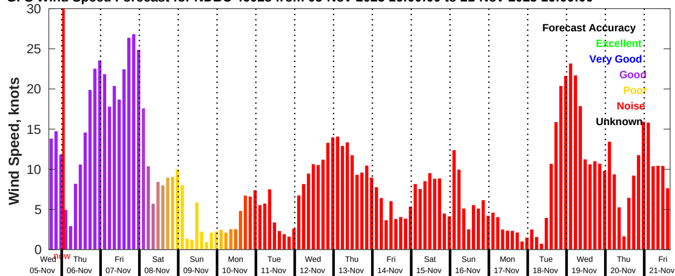
GFS Wind Speed Forecast for NDBC 46028 from 05-Nov-2025 16:00:00 to 21-Nov-2025 16:00:00
