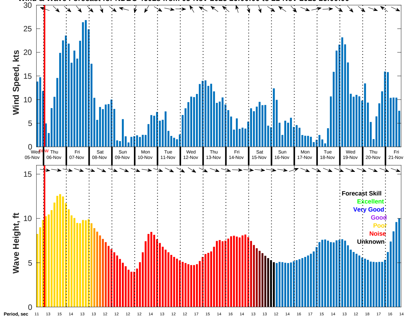
Wind & Wave Forecast for NDBC 46028 from 05-Nov-2025 16:00:00 to 21-Nov-2025 16:00:00
