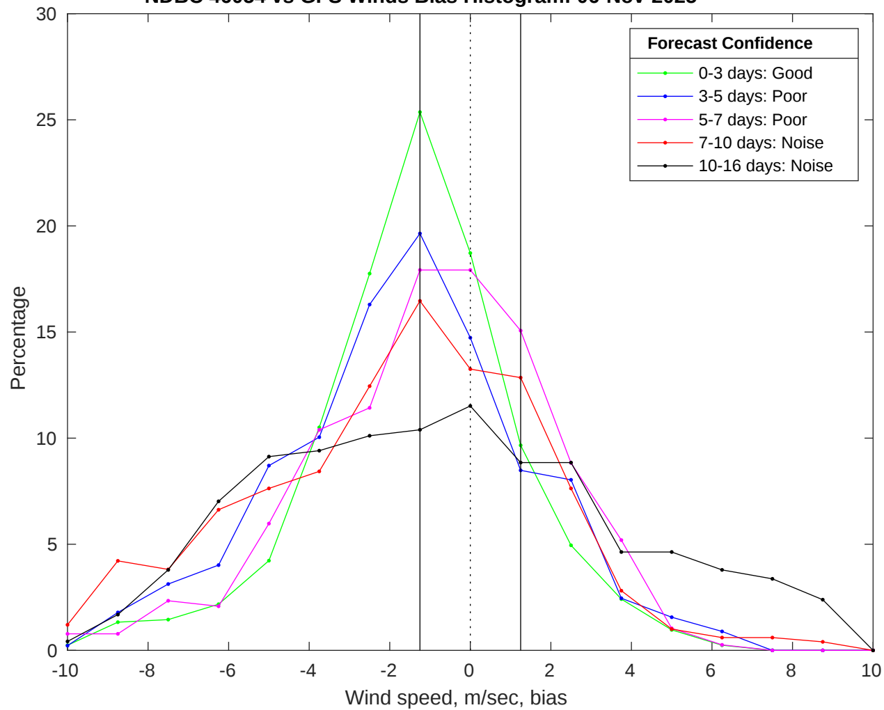
NDBC 46054 vs GFS Winds Bias Histogram: 06-Nov-2025
