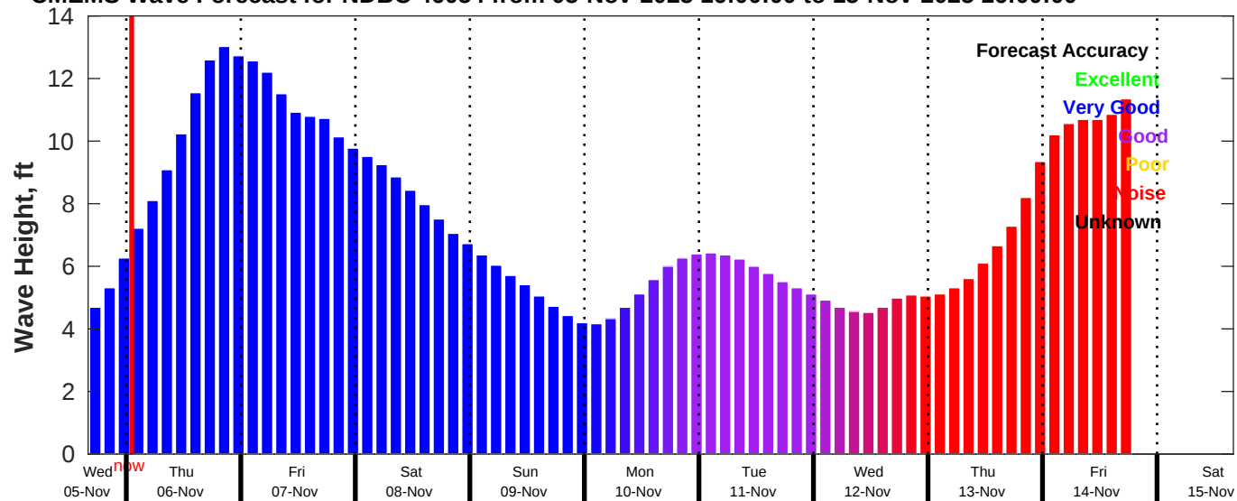
CMEMS Wave Forecast for NDBC 46054 from 05-Nov-2025 16:00:00 to 15-Nov-2025 16:00:00
