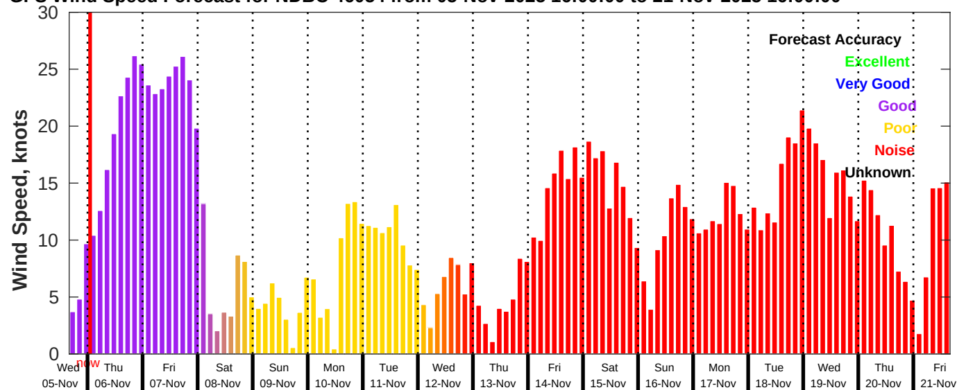
GFS Wind Speed Forecast for NDBC 46054 from 05-Nov-2025 16:00:00 to 21-Nov-2025 16:00:00
