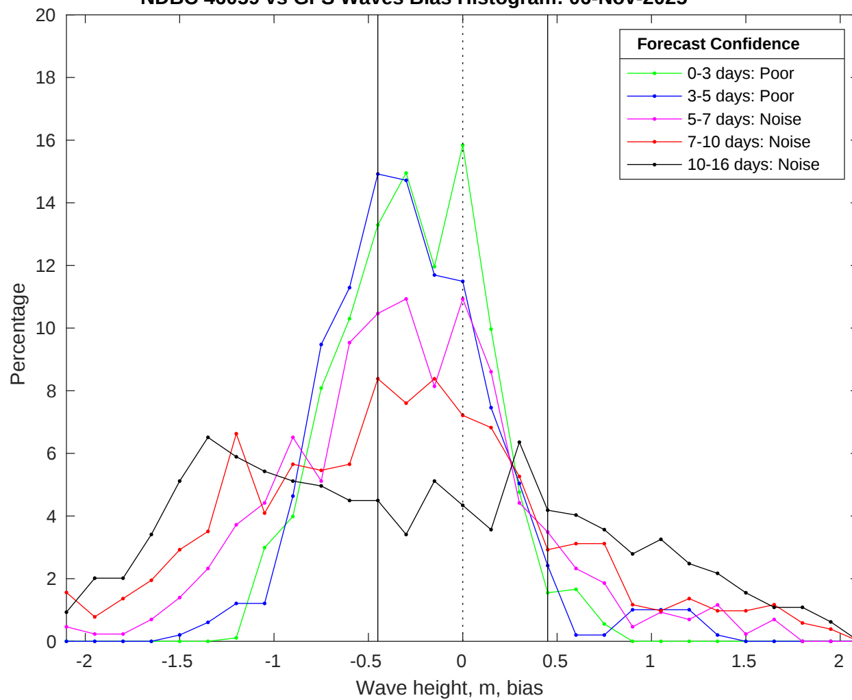
NDBC 46059 vs GFS Waves Bias Histogram: 06-Nov-2025
