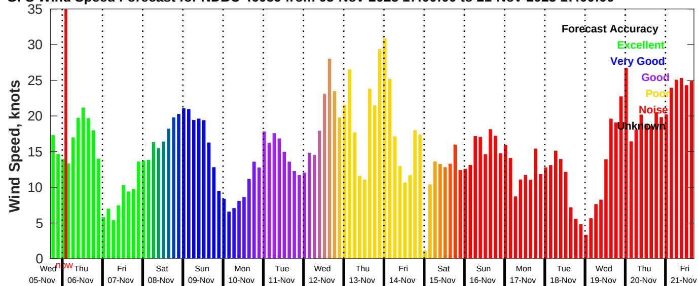
GFS Wind Speed Forecast for NDBC 46059 from 05-Nov-2025 17:00:00 to 21-Nov-2025 17:00:00
