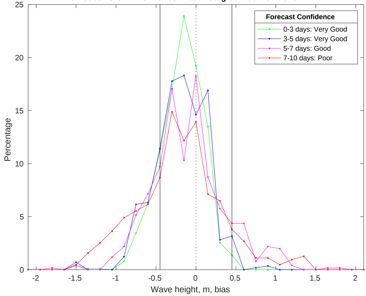
NDBC 46069 vs CMEMS Waves Bias Histogram: 06-Nov-2025
