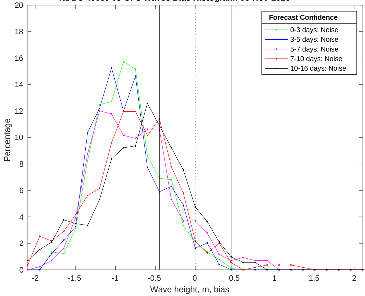
NDBC 46069 vs GFS Waves Bias Histogram: 06-Nov-2025
